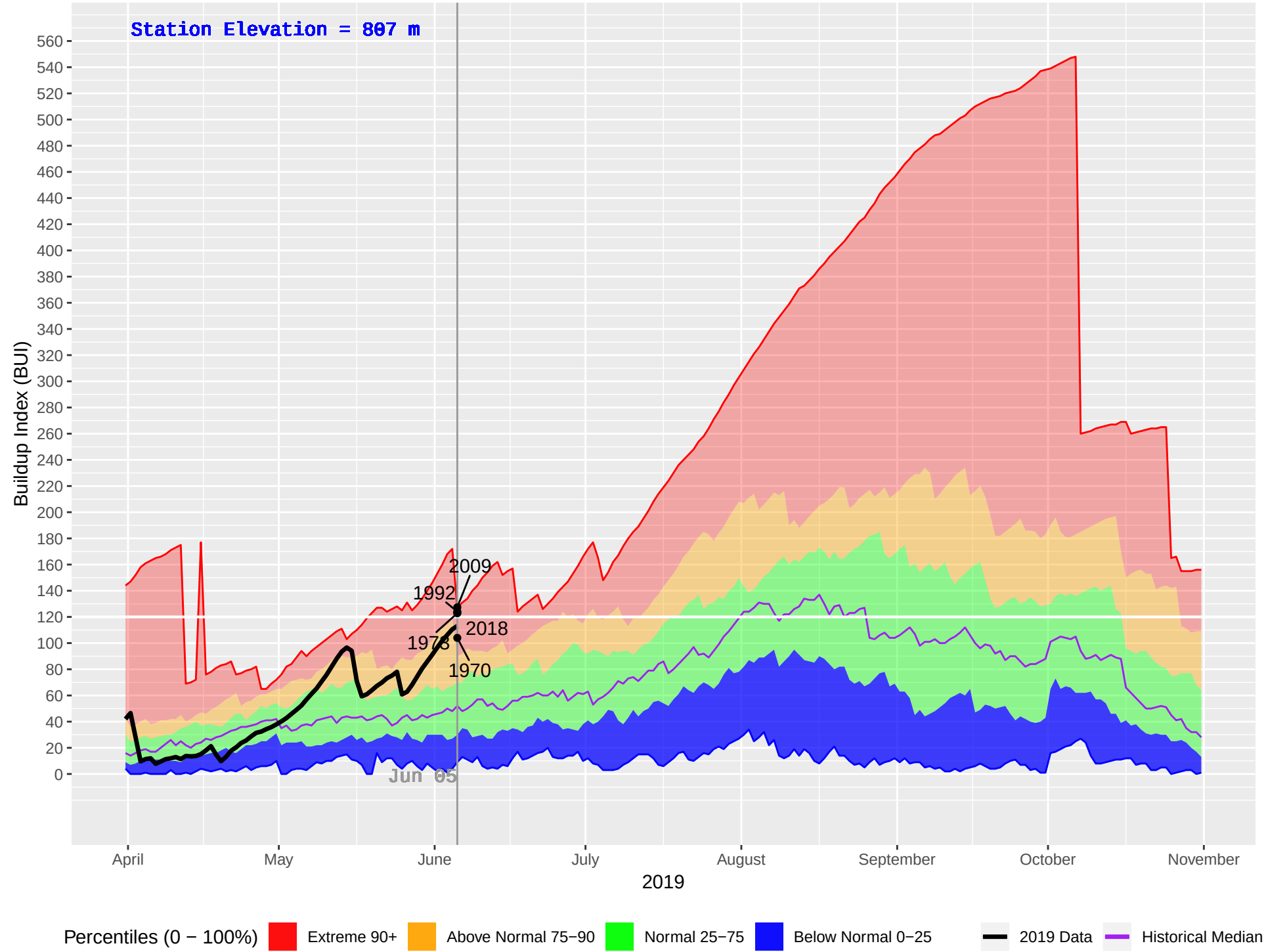
BEAVERDELL (390) : Historical (1970–2018), Current (2019) Daily Buildup Index (BUI)
