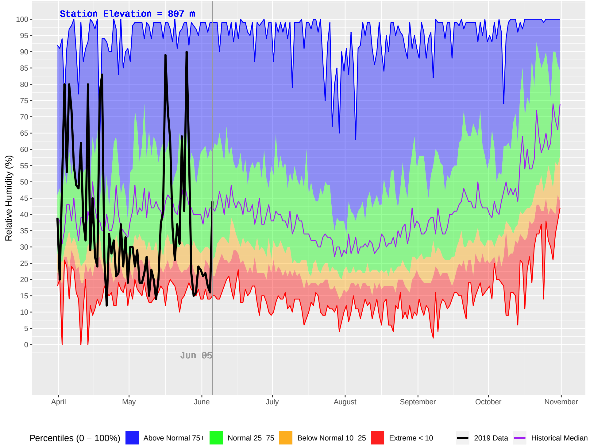
BEAVERDELL (390) : Historical (1970–2018) and Current (2019) Daily Relative Humidity
