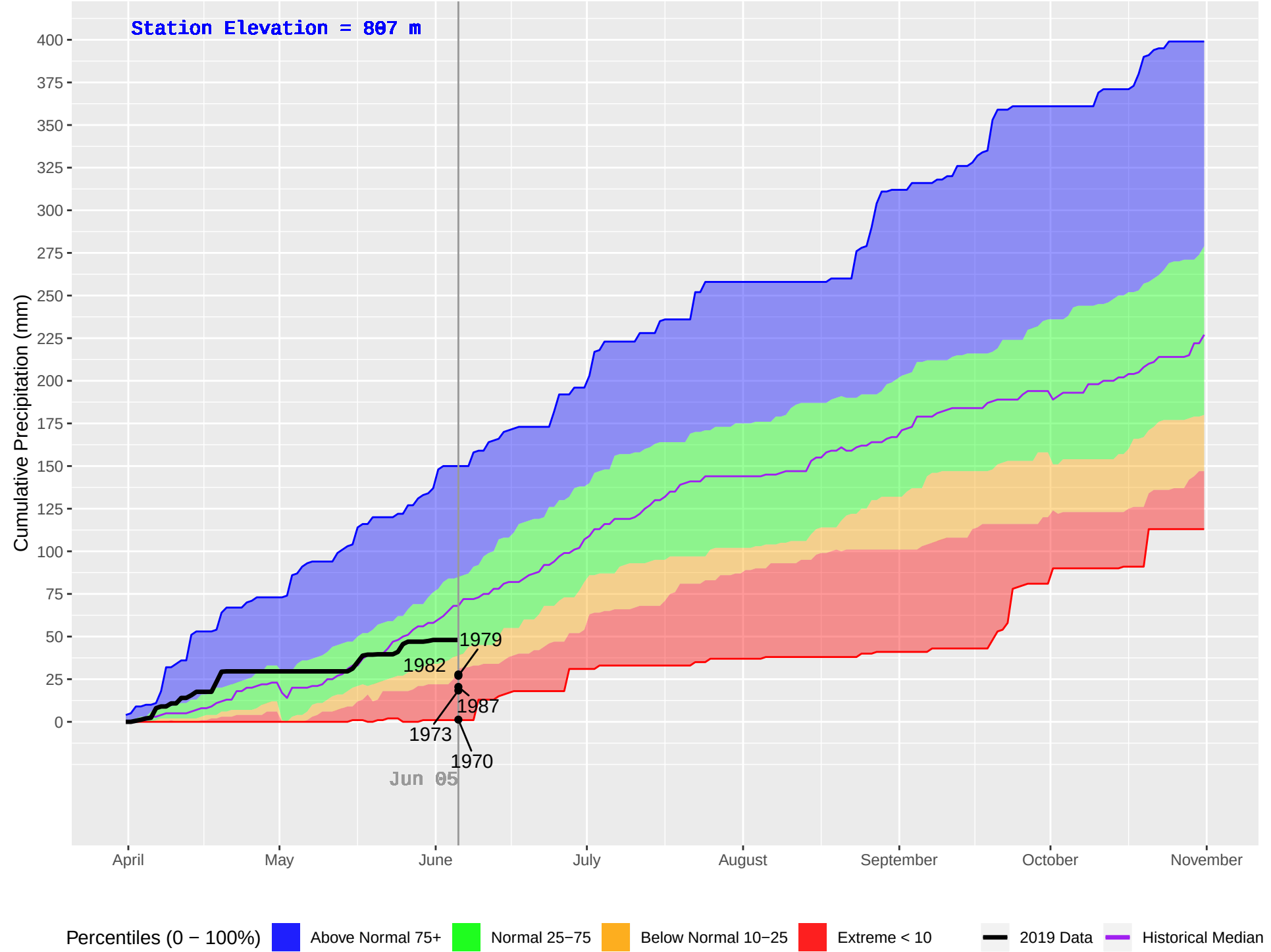
BEAVERDELL (390) : Historical (1970–2018), Current (2019) Daily Cumulative Precipitation
