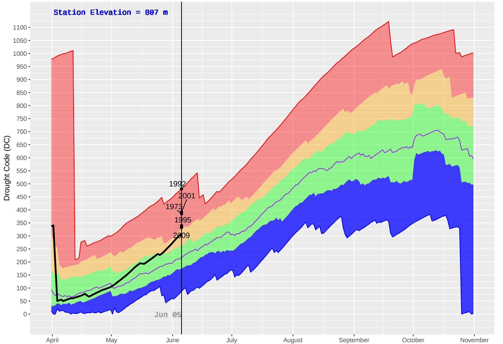
BEAVERDELL (390) : Historical (1970–2018) and Current (2019) Daily Drought Code (DC)
