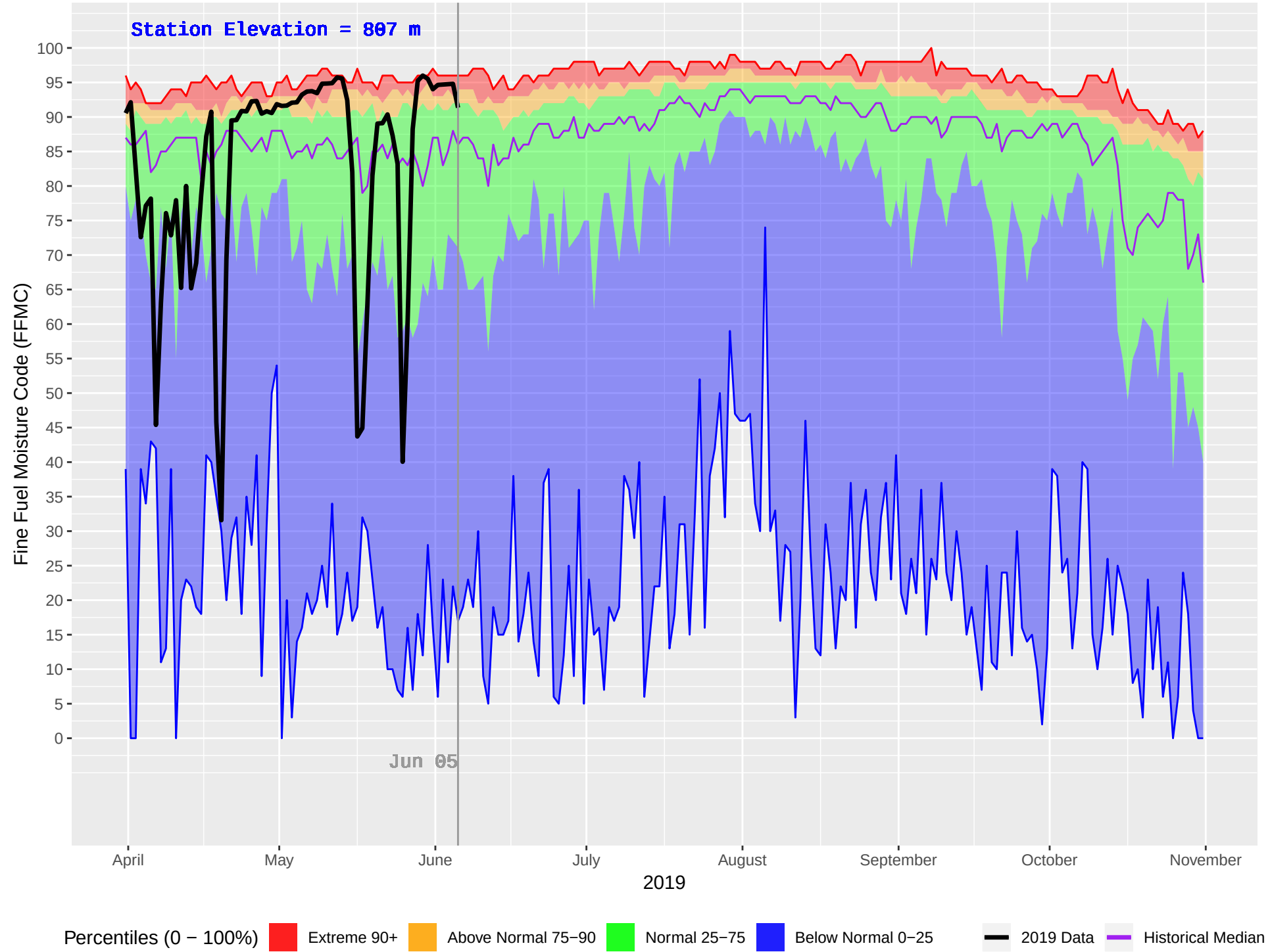
BEAVERDELL (390) : Historical (1970–2018) and Current (2019) Daily Fine Fuel Moisture Code (FFMC)
