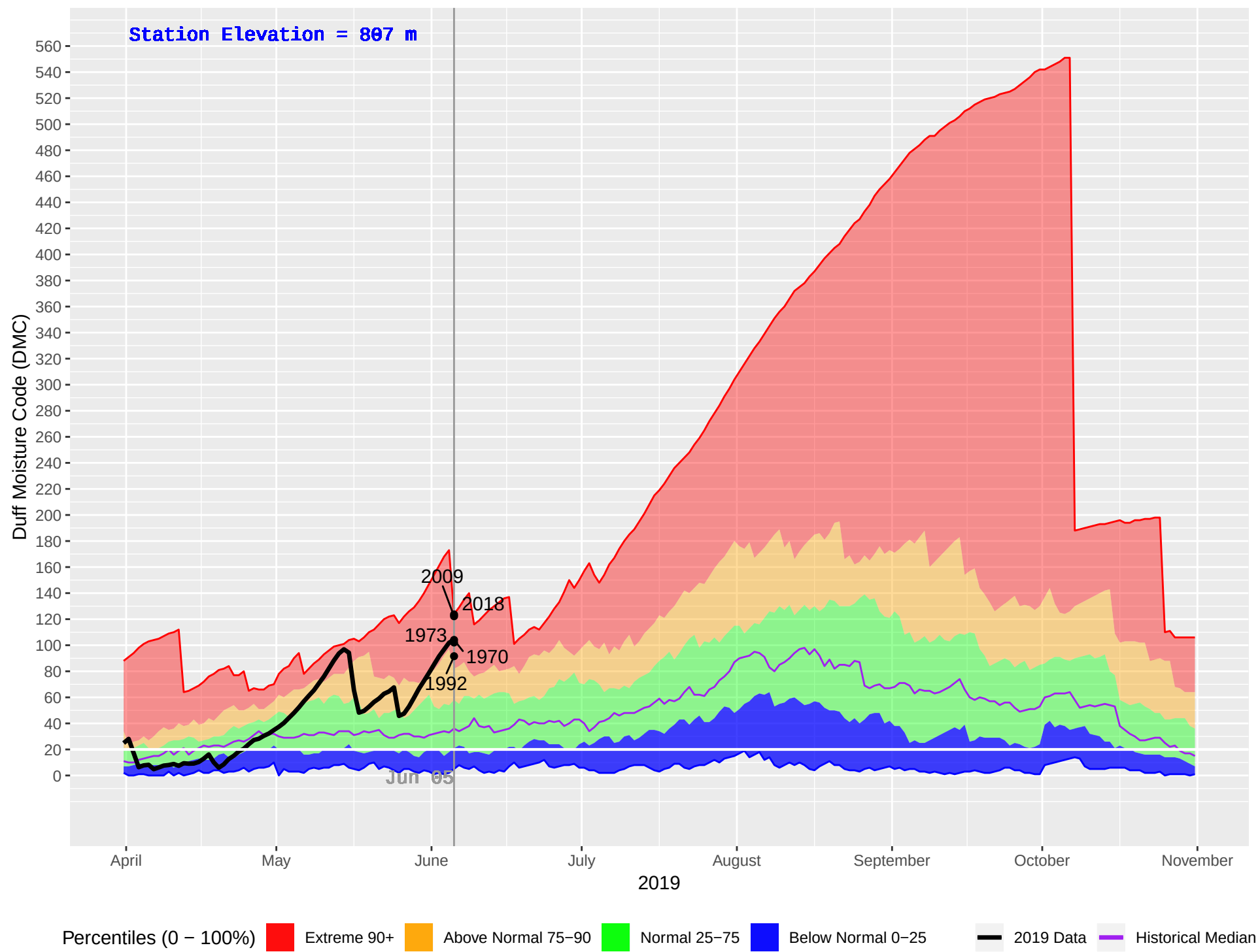
BEAVERDELL (390) : Historical (1970–2018), Current (2019) Daily Duff Moisture Code (DMC)
